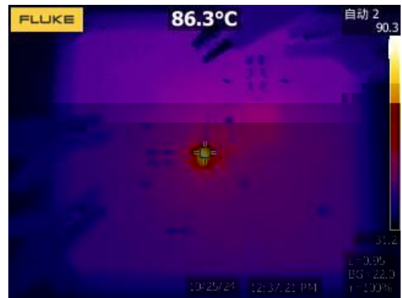
Figure 23. Thermal, 12VIN, 5Vout, 3A
