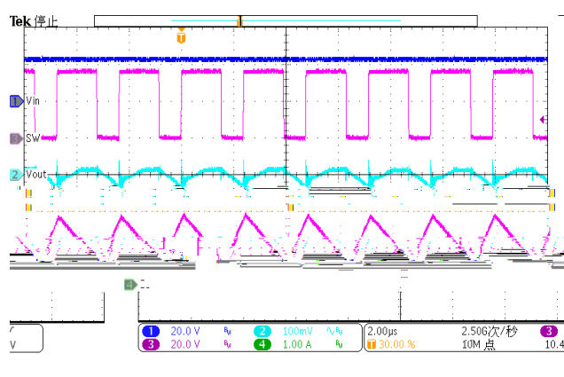
Figure 36. steady-state (Iload=2A)
