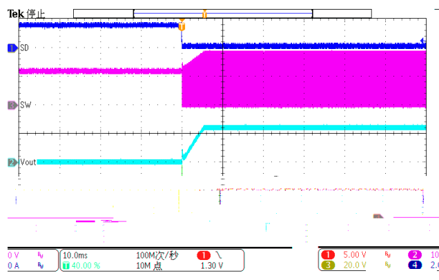
Figure 34. Shutdown remove
